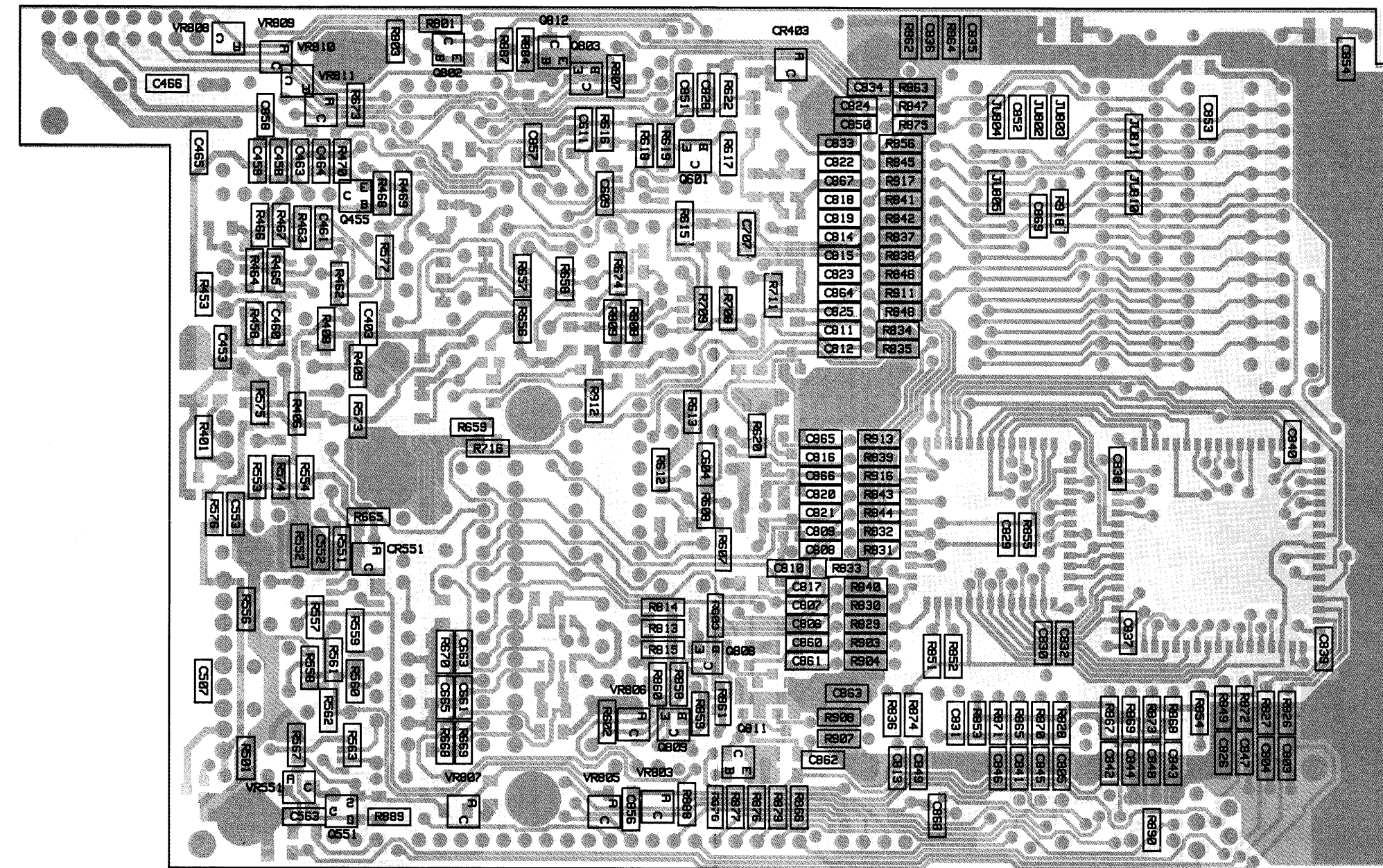
SOLDER SIDE
