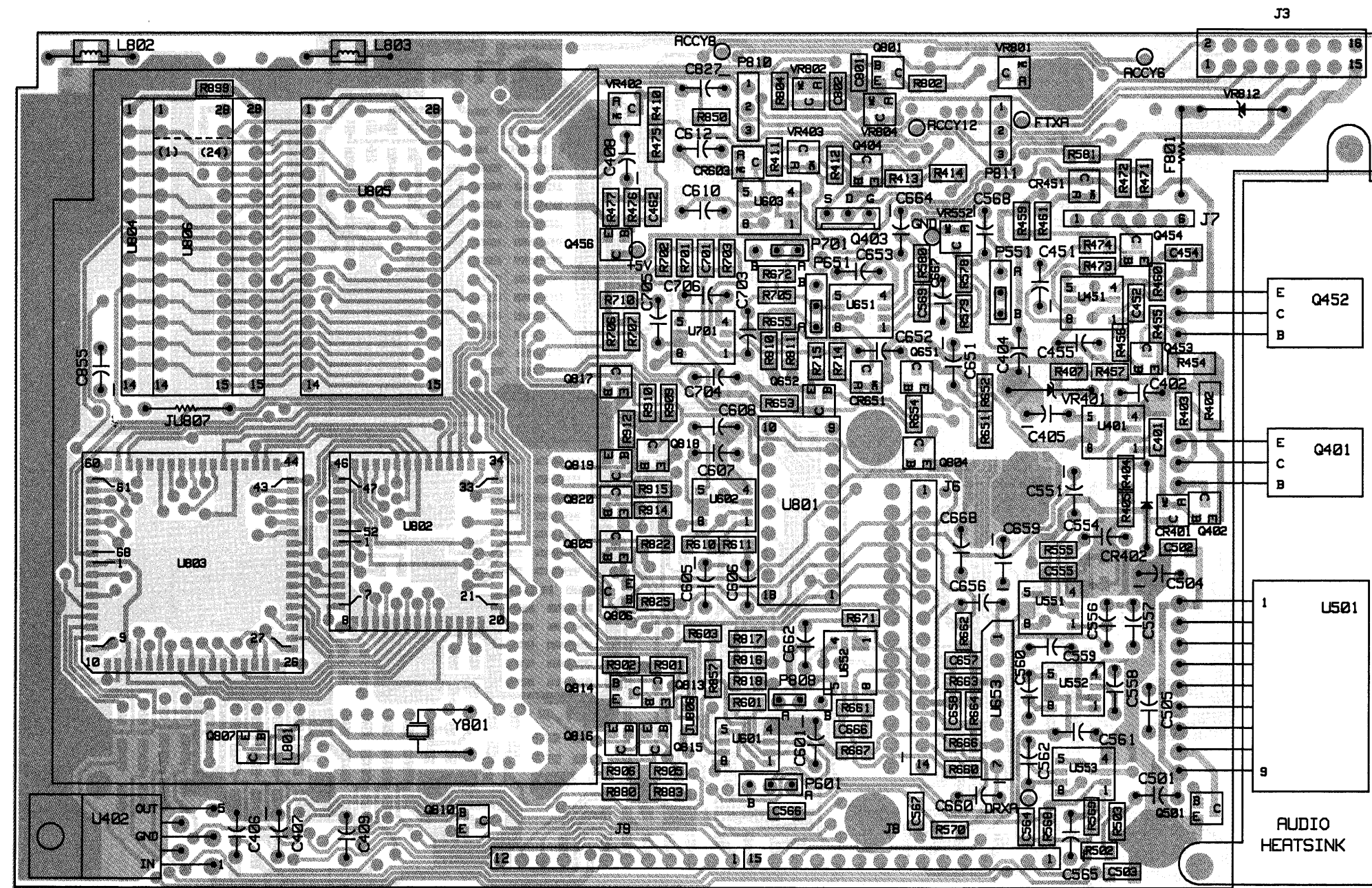
COMPONENT SIDE
