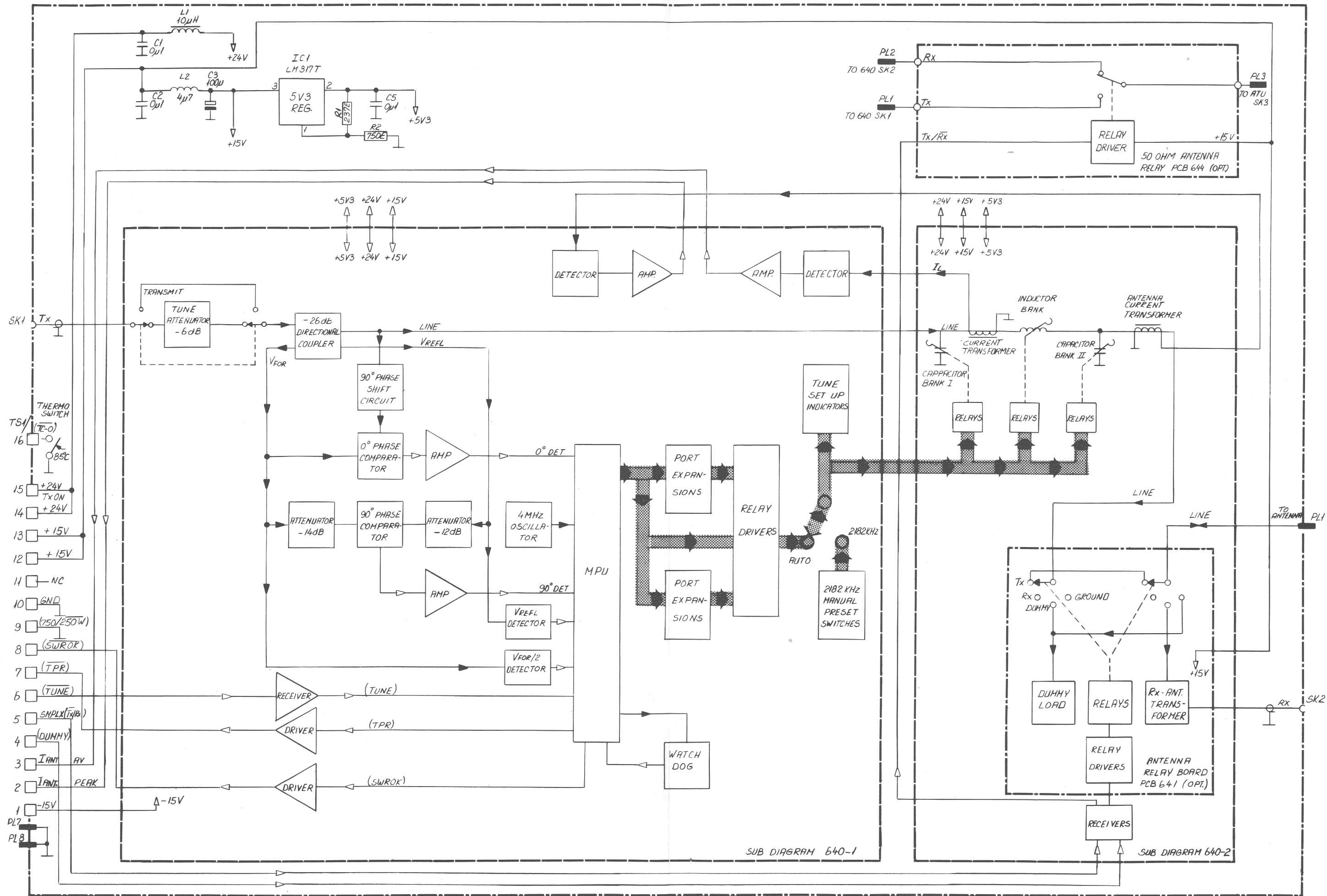
MAIN DIAGRAM ANTENNA TUNING UNIT 640 VERSION 4A
