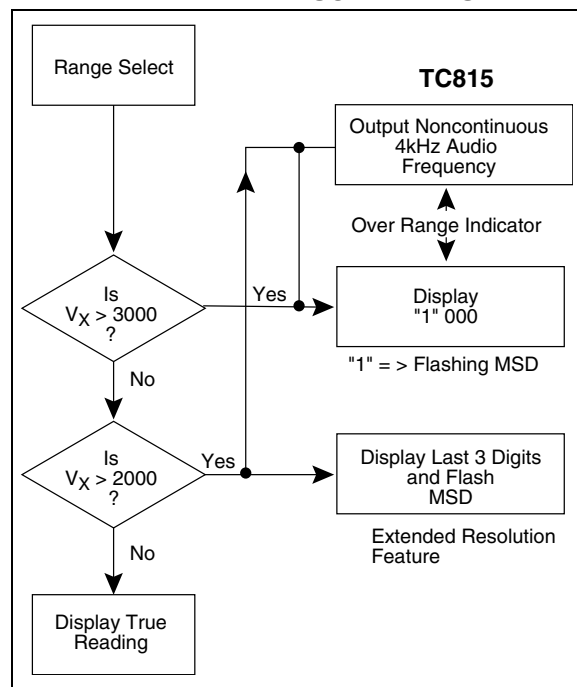
FIGURE 5-3: MANUAL RANGE SELECTION: VOLTAGE MEASUREMENTS
